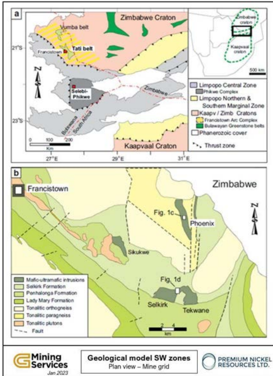
Figure 7-1: a) Schematic Map of Limpopo Belt and Adjacent Cratons Showing Studied Localities b) Geological Map of the Central Portion of the Tati Greenstone Belt Indicating Locality of Phoenix, Selkirk and Tekwane Deposits
