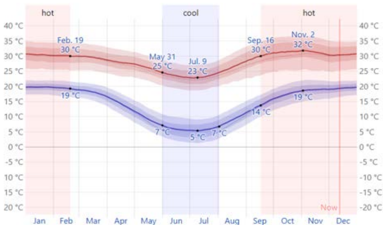
Figure 5-1: Average Annual Temperatures at Francistown Airport
