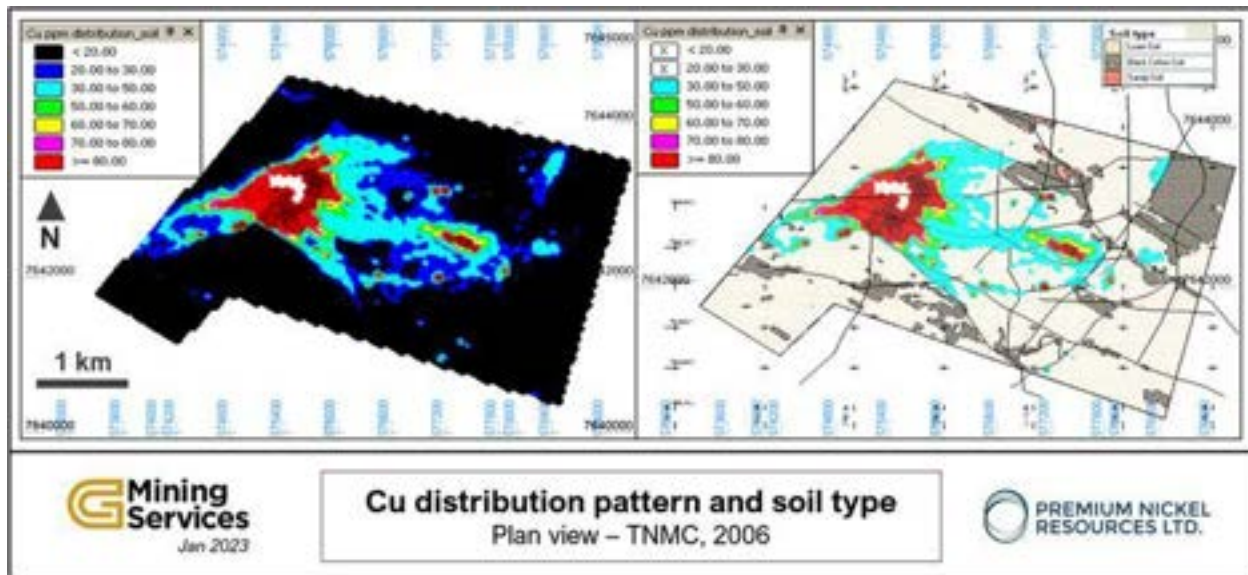
Figure 9-6: a) Distribution Pattern Showing Concentrations of Cu at Selkirk. b) Cu Concentrations Superimposed with Soil Type and Geological Structures.
