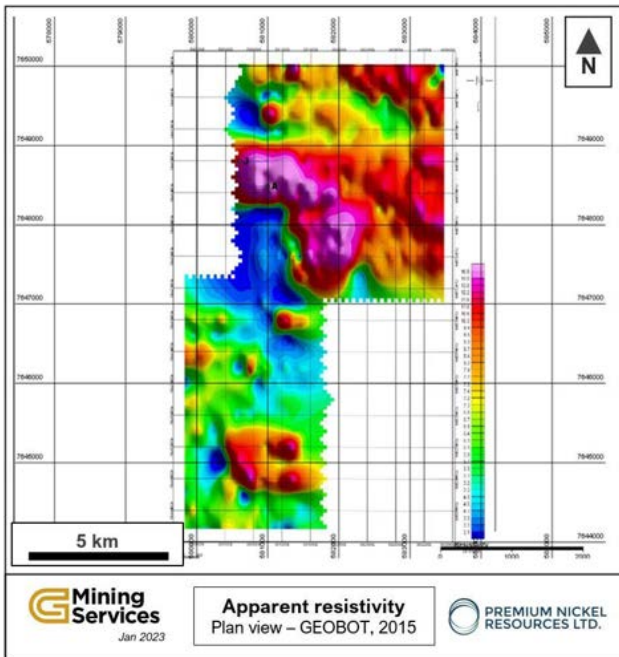
Figure 9-13: Prospect PL071/2011 IP Geophysical Survey
