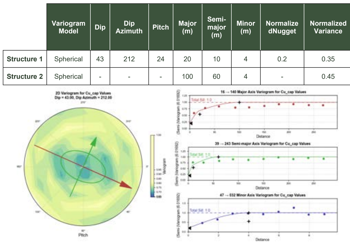
Figure 14-5: Copper Variogram Map and Model Results for the Upper Domain - Selebi
