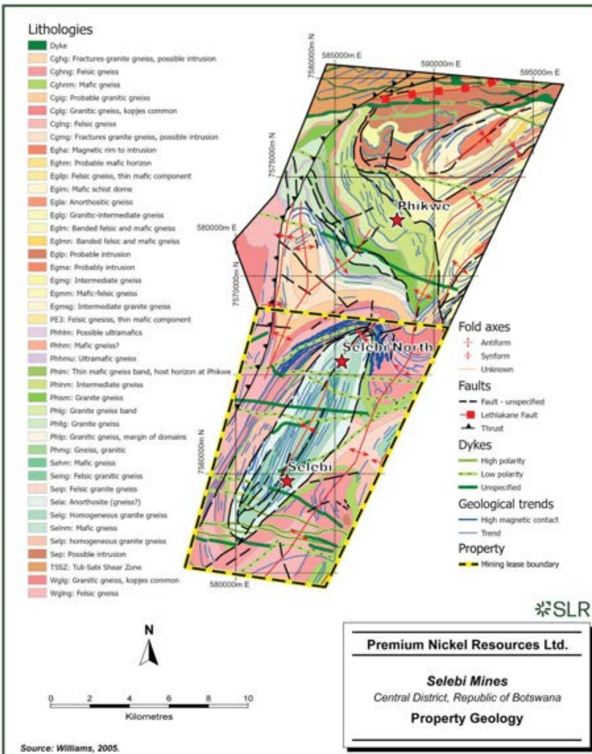
Figure 7-5: Property Geology
