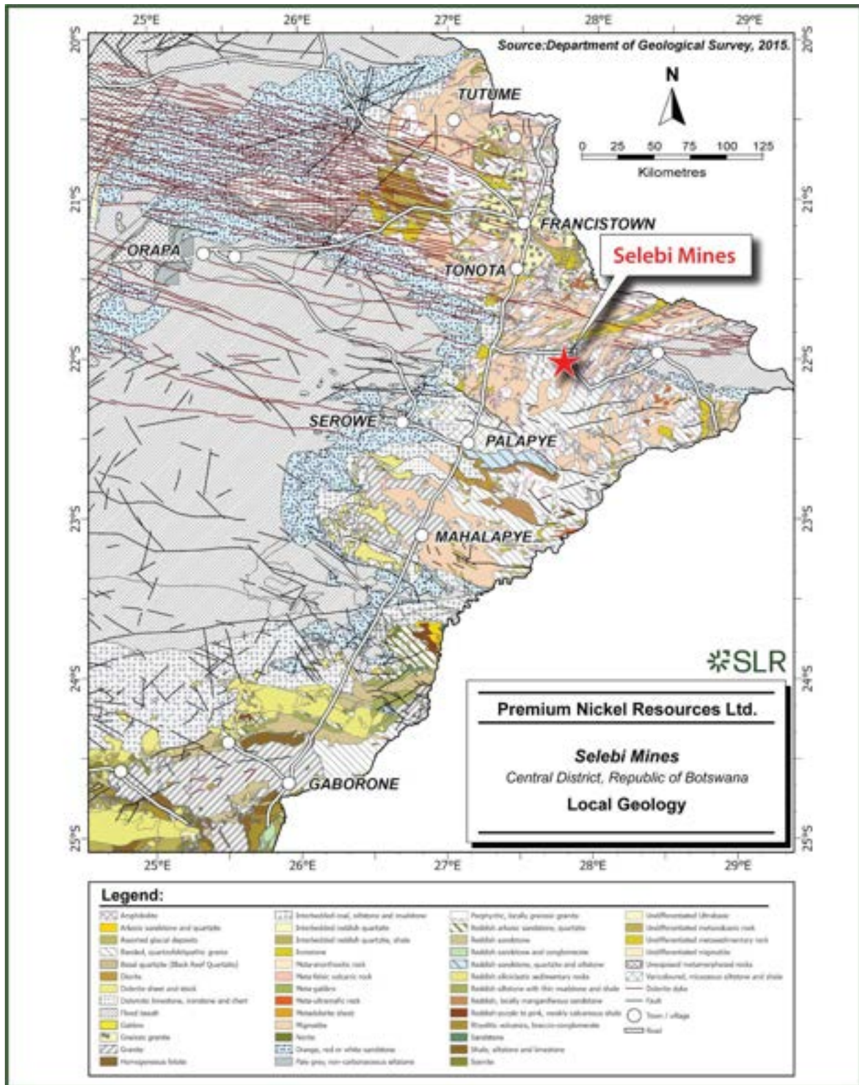
Figure 7-2: Local Geology
