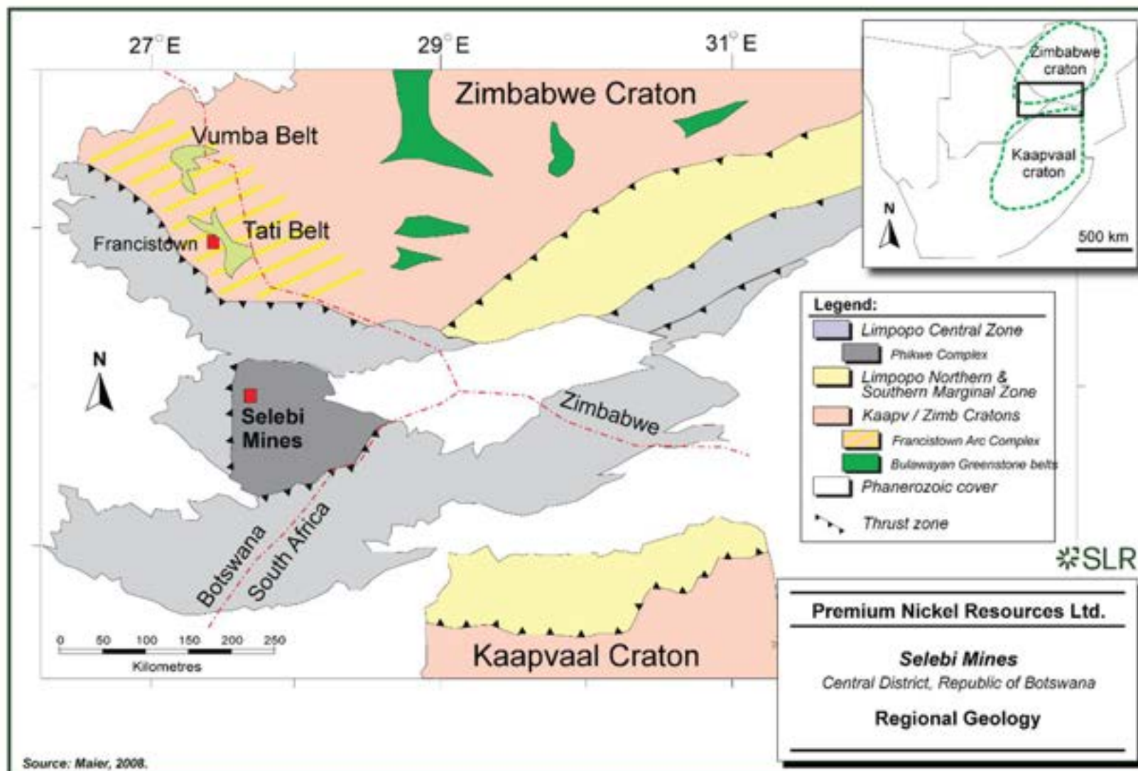
Figure 7-1: Regional Geology
