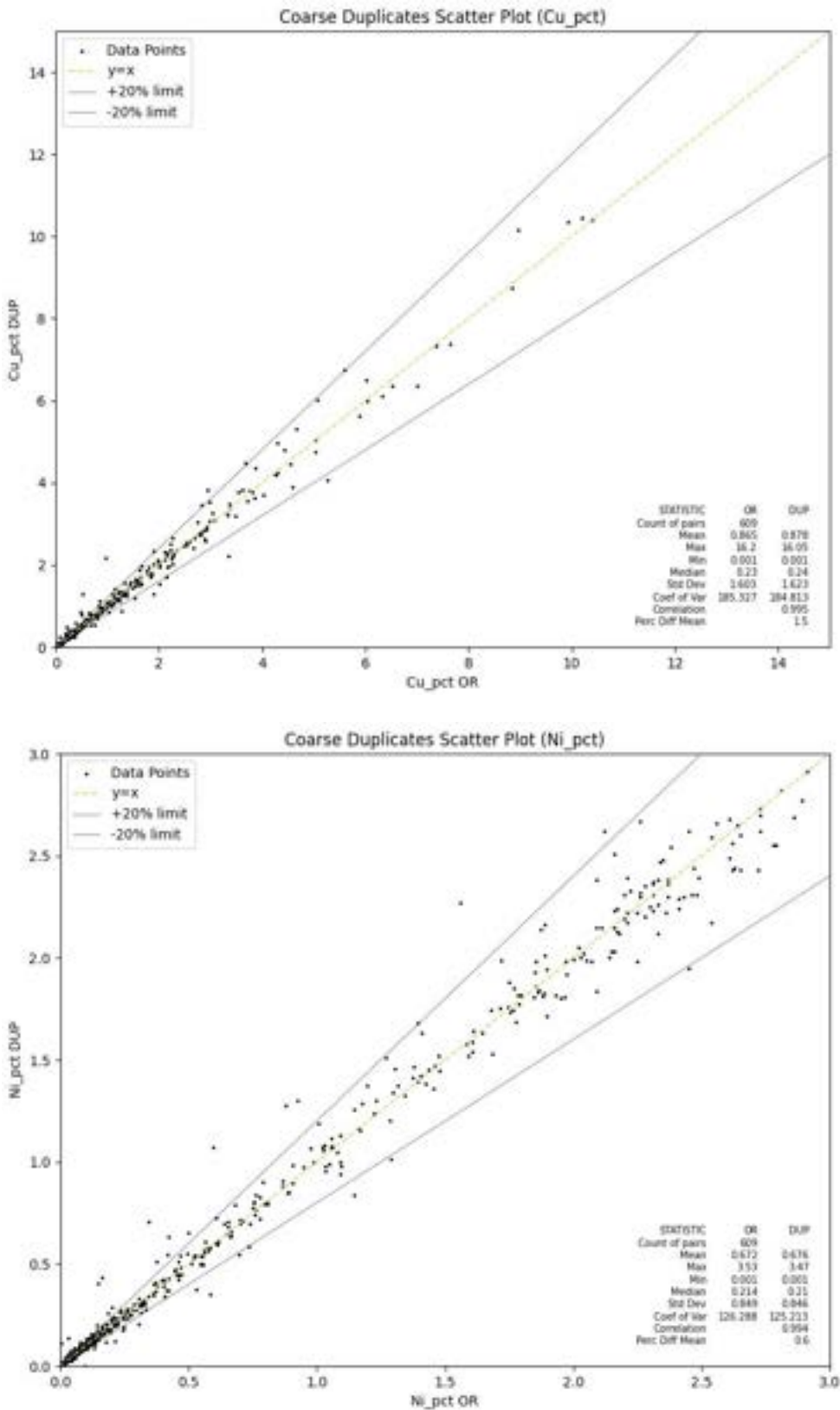
Figure 11-5: Selebi Scatter Plots of Coarse Duplicates at ALS: 2022 to 2024
