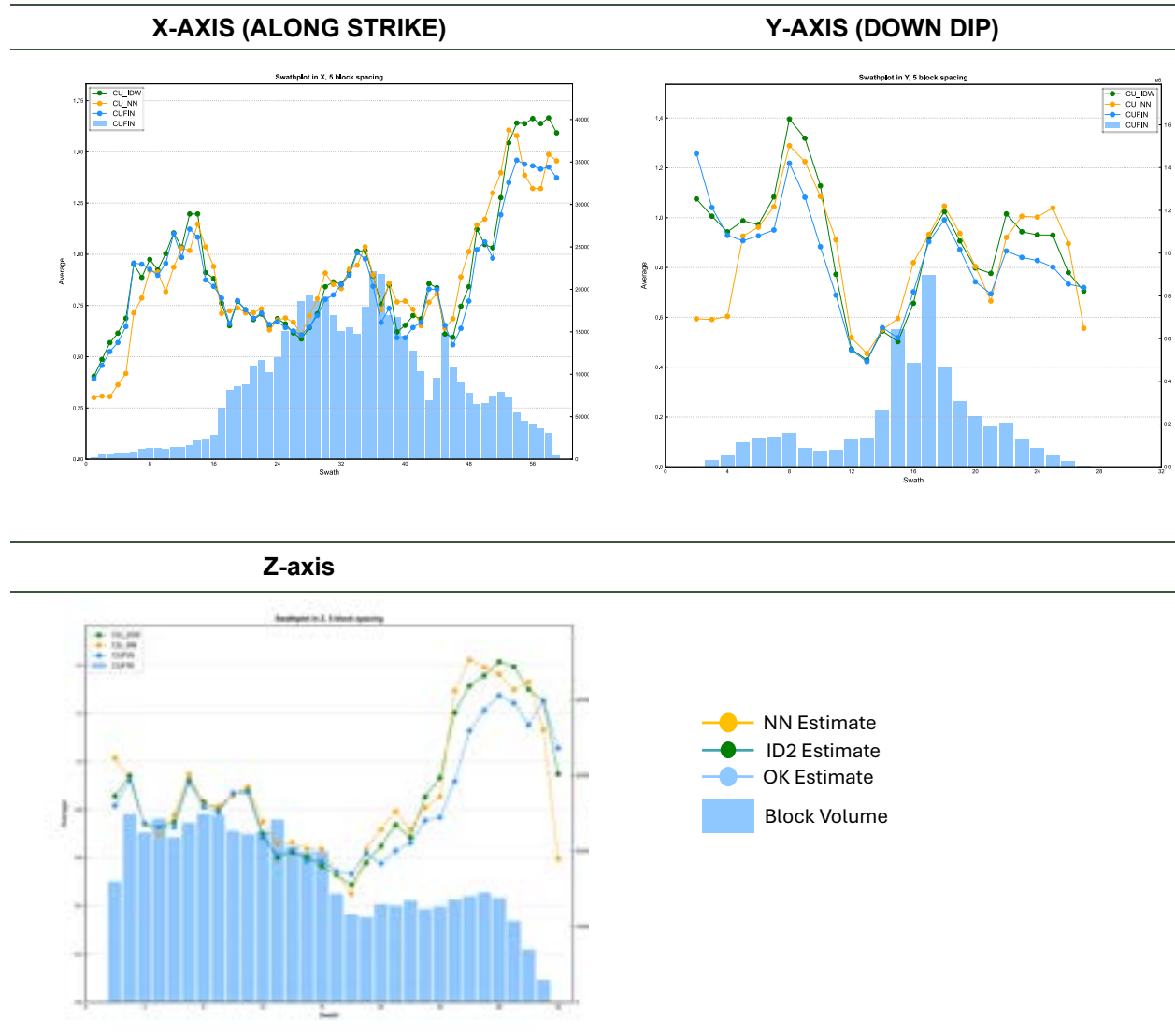
Figure 14-21: Comparison between OK, ID, and NN Mean Swath Plots for Copper in the Main Domain – Selebi North
